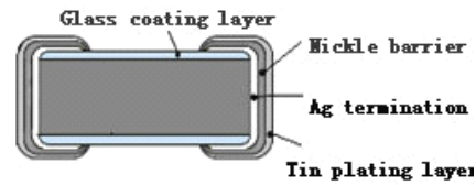
Side section
